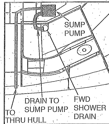
FWD HEAD SHOWER DRAIN
