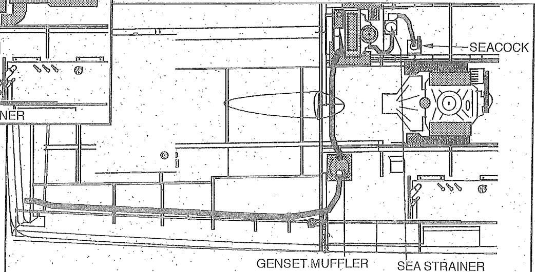
GAS ENGINE
