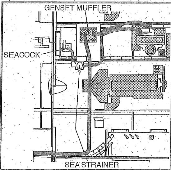
DIESEL ENGINE
