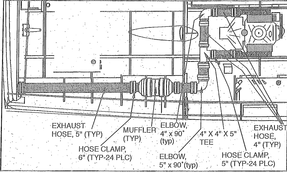
GAS ENGINE
