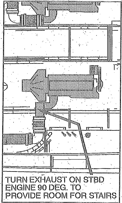
DIESEL ENGINE
