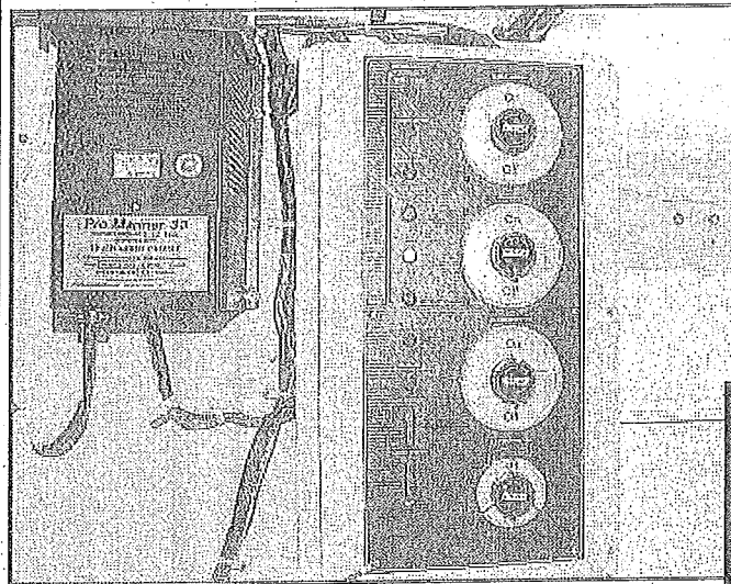
THE BATTERY SWITCHES AND THE BATTERY CHARGER ARE LOCATED ON THE AFT ENGINE ROOM BULKHEAD, NEXT TO THE COCKPIT-TO ENGINE ROOM ACCESS DOOR
